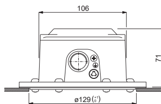
SMALL FLANGE
