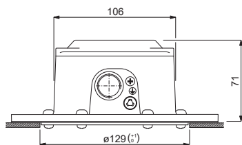
STANDARD FLANGE
